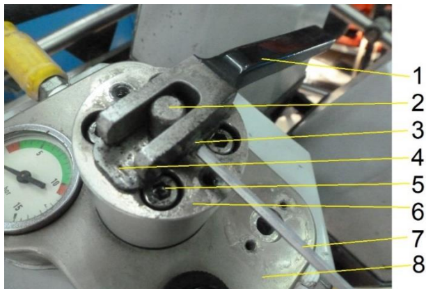
Fig. 1: Main blast valve view
